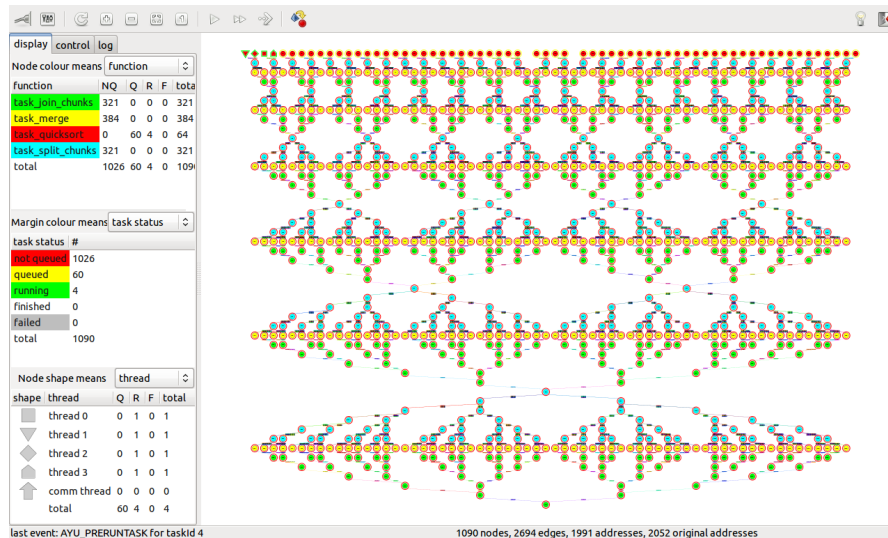
Figure 2: TEMANEJO screenshot
