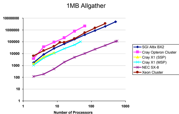
Figure 10: Execution time of Allgather benchmark on varying number of processors, using a message size of 1MB, in \mu\text{s/call} (i.e., the smaller the better).
