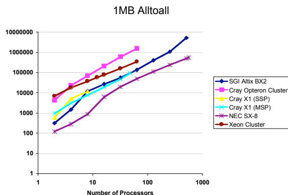
Figure 12: Execution time of AlltoAll benchmark on varying number of processors, using a message size of 1MB, in \mu\text{s/call} (i.e., the smaller the better).
